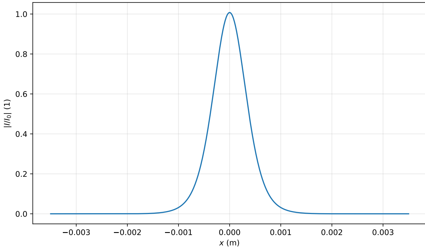
Intensity profile I(x, y = 0, z = 1.751m)/I_0 , P_{in}=0.6P_{cr} , artificial time
